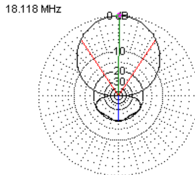
Free-Space 17-Meter E-Plane Pattern
