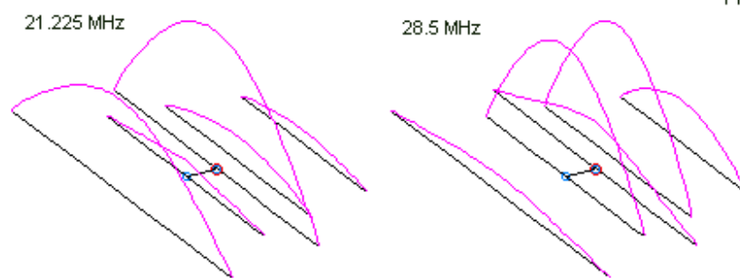
Relative Current Magnitude Distribution: 5-Element 2-Band Array
