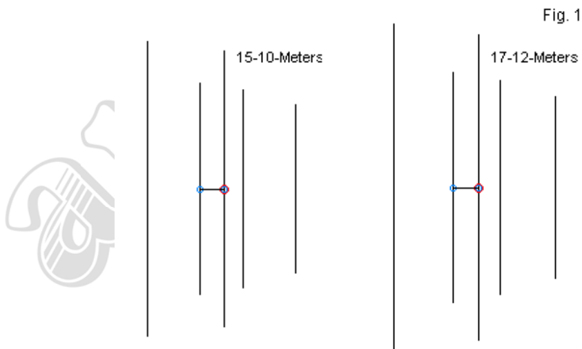
General Outlines: 5-Element Yagi-Yagi Beams for 15-10-Meters and 17-12-Meters
