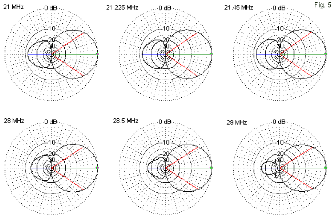
Free-Space E-Plane Patterns: 15-10-Meter 5-Element Array
