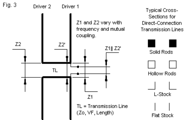
Feedpoint Considerations for Directly Connected Drivers
