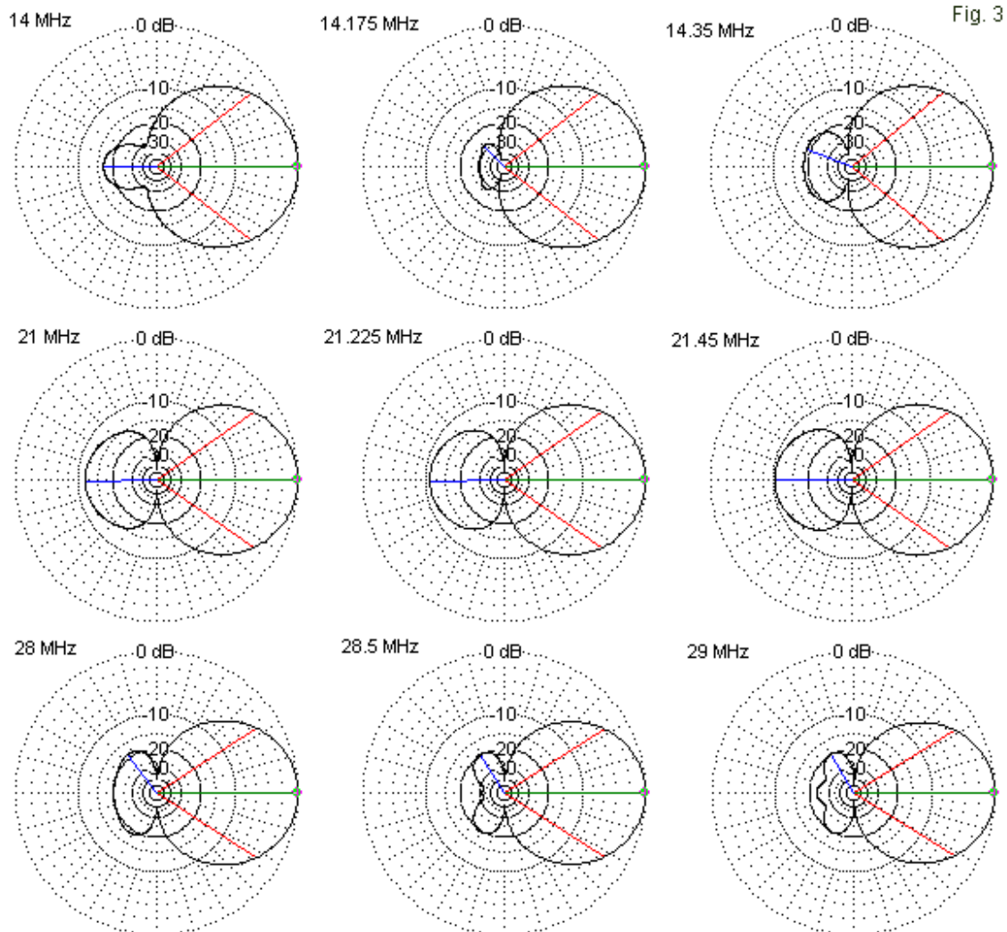
Selected Free-Space E-Plane Patterns: Type-1 Tri-Band Array 10-Meter Driver Rearward, 50-Ohm Feedpoint Connection Line, Cable to 20-Meter Element
