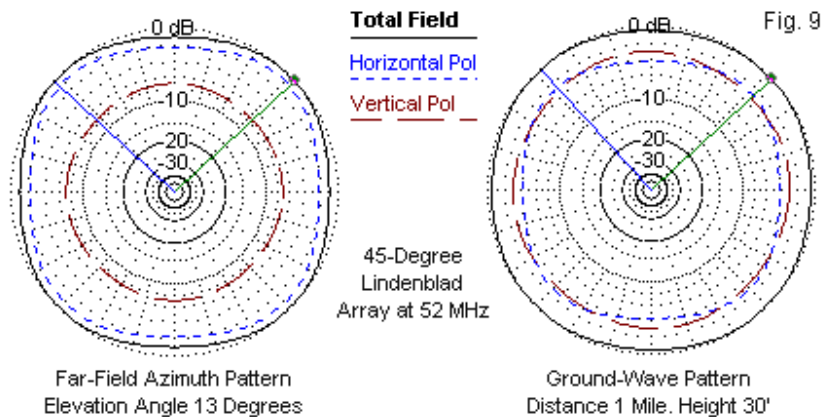
Vertical and Horizontal Components of Far-Field and Ground-Wave Patterns
