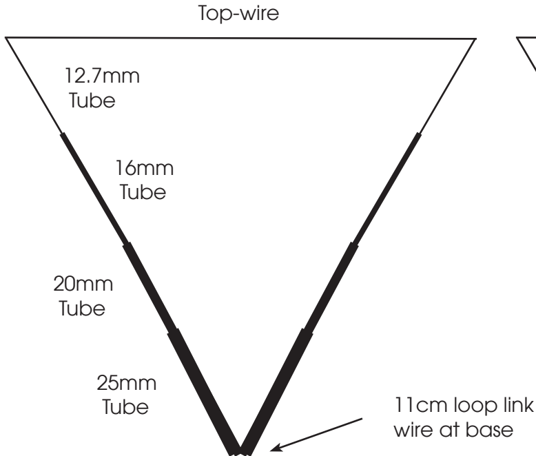
Reflector Element
