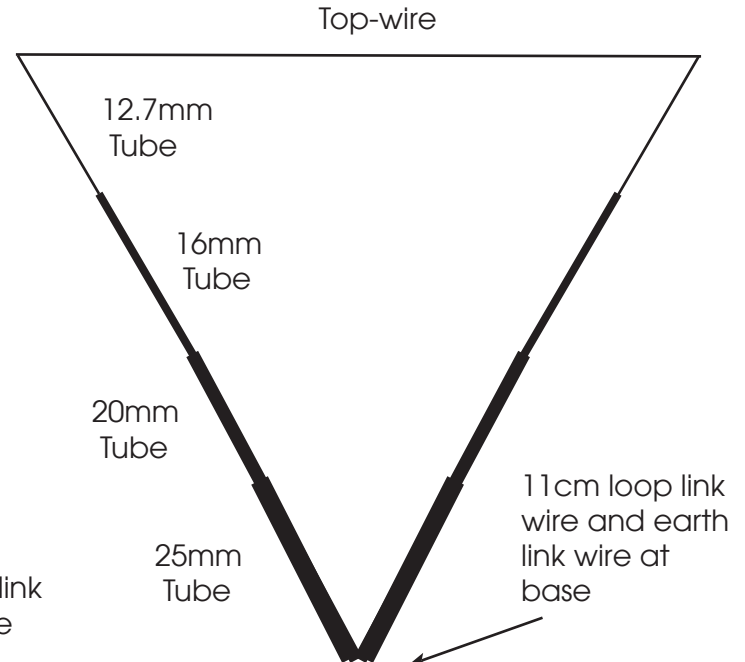
Driven Element
