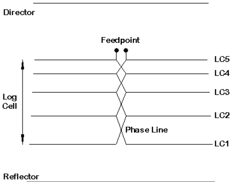
Fig. 5-1 Components of a Monoband Log-Cell Yagi
