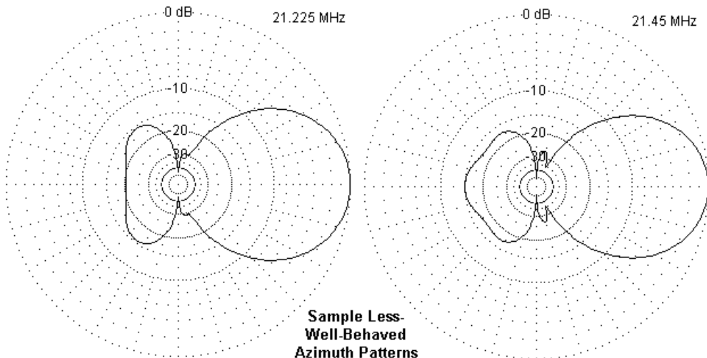
Fig. 17. Samples of less well-behaved free-space azimuth patterns from 15 meters.
