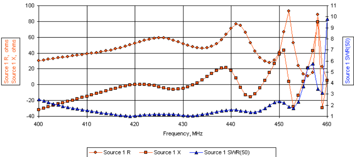
DL6WU 16 elements (Pattern Data: Az at 0° EI)
