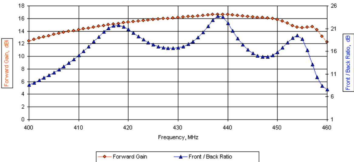
DL6WU 16 elements (Pattern Data: Az at 0° EI)
