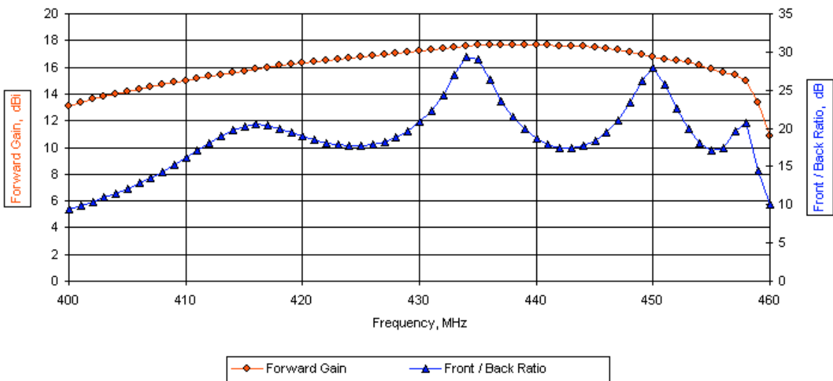
DL6WU 20 elements (Pattern Data: Az at 0° EI)
