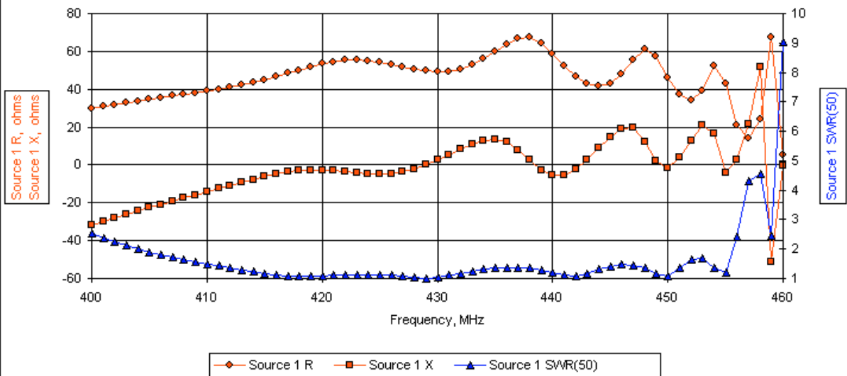
DL6WU 20 elements (Pattern Data: Az at 0° EI)
