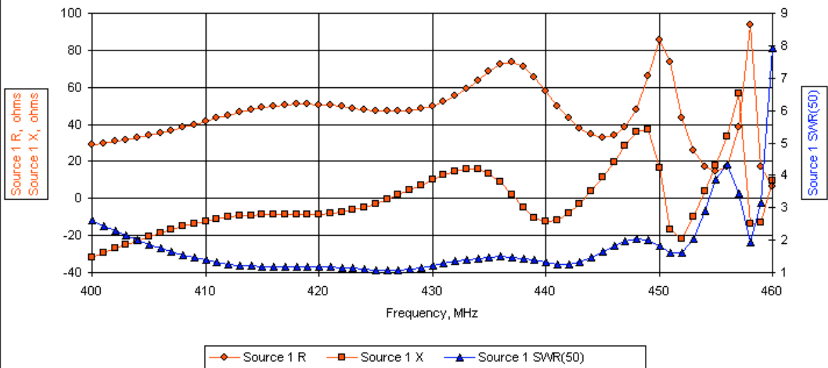
DL6WU 14 elements (Pattern Data: Az at 0° EI)
