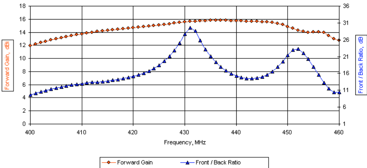
DL6WU 14 elements (Pattern Data: Az at 0° EI)
