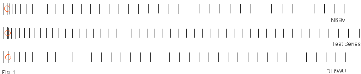
Comparative Outlines: DL6WU and N6BV 40-Element Yagis and Test Series 50-Element Yagi (Arrays To Scale)
