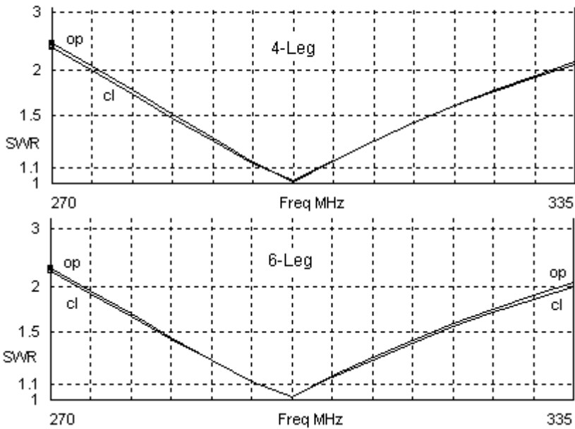
SWR Bandwidths Referenced to Resonant Impedance 4- and 6-Leg Biconical Models Using Multiple Center Wires Open-End and Closed-End Versions
