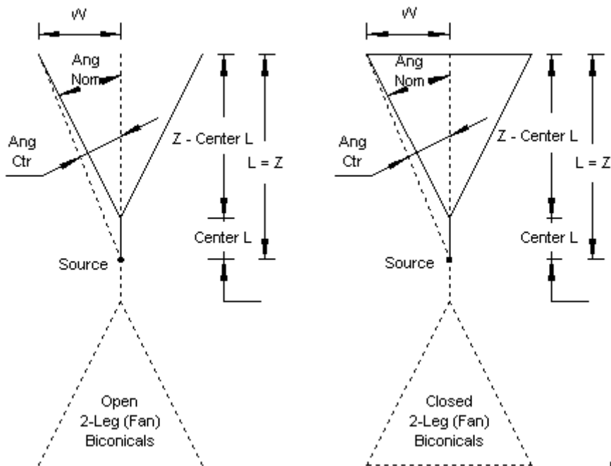
Guide to Tabular Dimension Listings for Open and Closed Biconical (Fan) Dipoles
