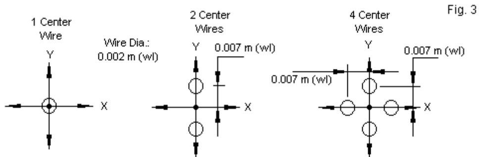
Model Layouts for Different Center-Wire Arrangements Looking Down (or Up) Z-Axis
