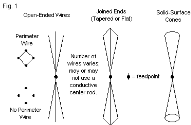
Some Biconical Configurations Used at VHF and UHF
