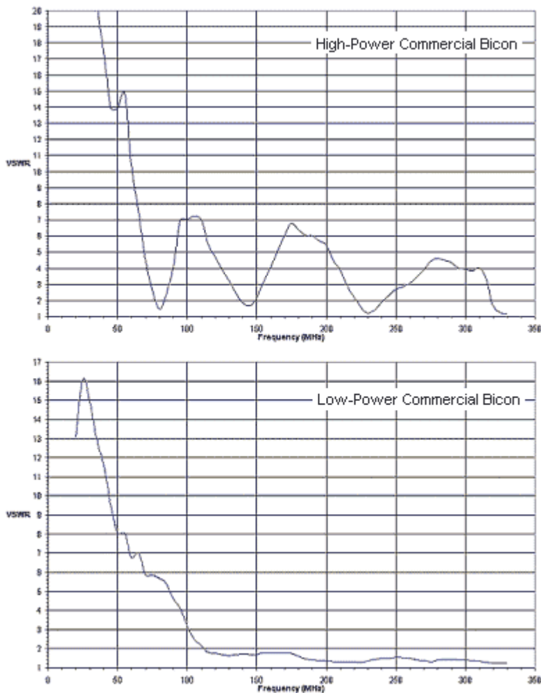
Typical Commercial Biconical Antenna SWR Curves
