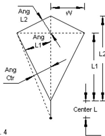
Guide to Tabular Dimension Listings for Tapered Closed Biconical (Fan) Dipoles
