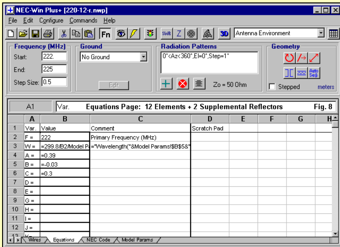
Fig. 8 shows the very simply equations page, with 3 variables, A, B, and C. A is the element half length in meters (the default unit of .NEC-format conversion from EZNEC to NEC-Win). B is the distance along the Y-axis, where a value of zero would align the new reflectors with the old. C is the vertical separation of each reflector above and below the plane of the other elements.
