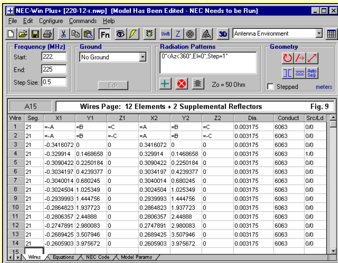
The wires page, Fig. 9 , shows the variable placement for the two new elements. The element length coordinates appears as A and -A. Likewise, the upper and lower new reflectors are at C and -C. Note that in this initial exercise, I did not alter the placement of length of the original reflector. In a full scale study, one might wish to convert this element to a set of variables and adjust its specifications. (Since the original reflector was crucial to obtaining the impedance curves across the passband, I left it unchanged as the simplest means of sustaining those curves.)
