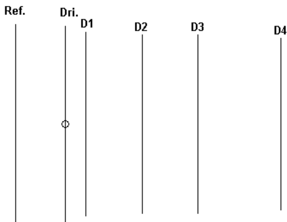
6-Element 2-Meter OWA Yagi
