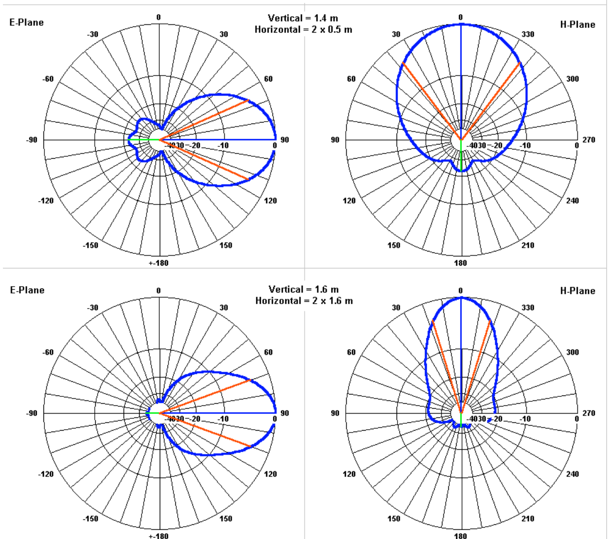
Fig. 17 Extremes of Corner-Reflector + Dipole Maximum Gain Free-Space Patterns Reflector Aperture = 1.414 \times Single Horizontal Dimension
