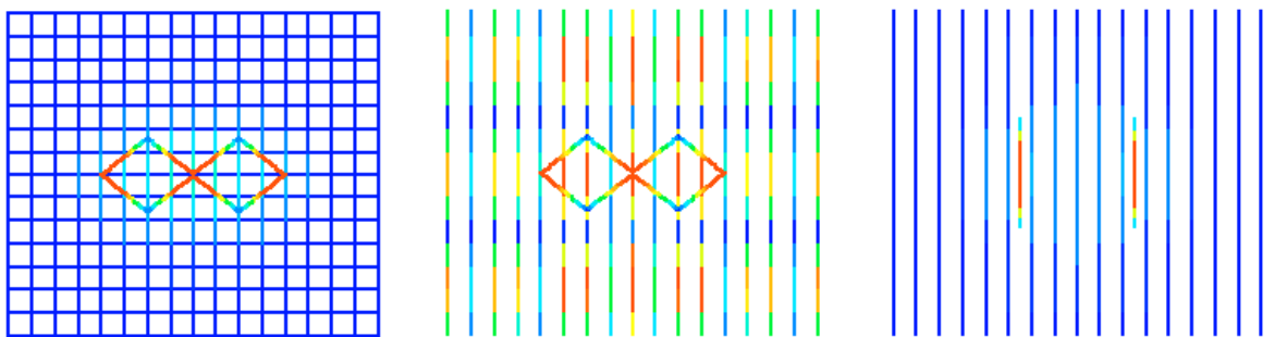
Current Distribution for a Double Diamond Driver with Wire-Grid and Rod Reflectors and for a Dual-Dipole Driver with a Rod Reflector
