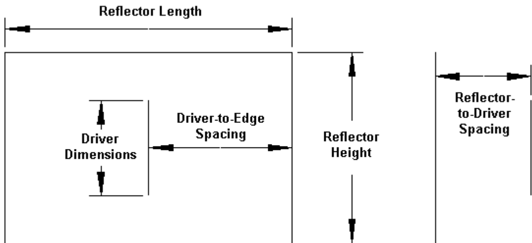
Planar Array Critical Dimensions
