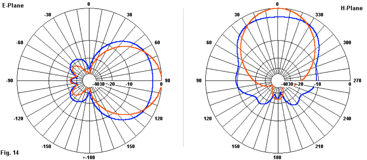
Comparative Free-Space Patterns Using 1.4-WL (V) by 1.2-WL (H) Reflectors Single Side-Fed Rectangle with Bar and Wire-Grid Reflectors
