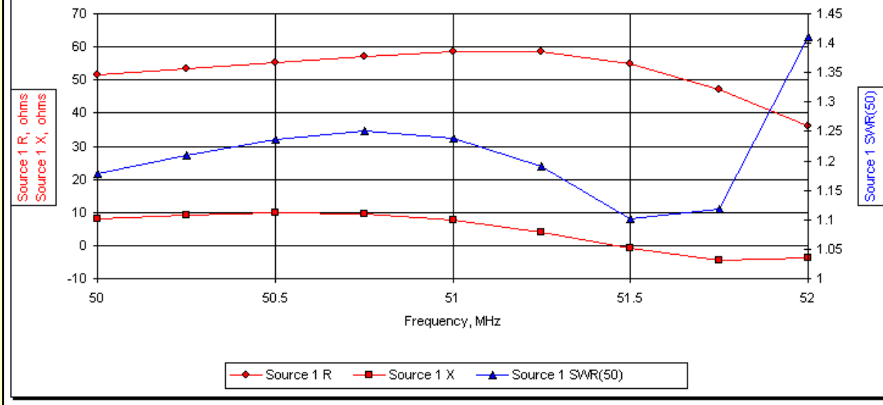
6m Yagi 0.625/0.5" Elements
