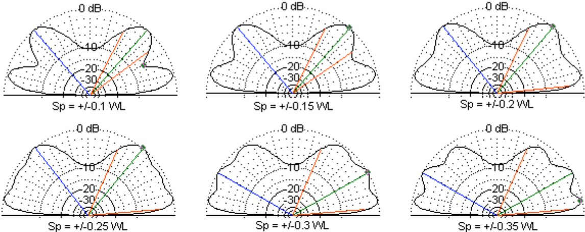
Lindenblad Elevation Patterns at 1 \text{ WL} above Average Ground Using Variable Spacing Between Facing Dipoles
