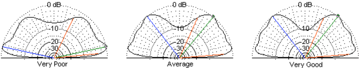
Lindenblad Elevation Patterns at 1 \text{ WL} above Various Ground Qualities Using \pm 0.25\text{-WL} Spacing Between Facing Dipoles
