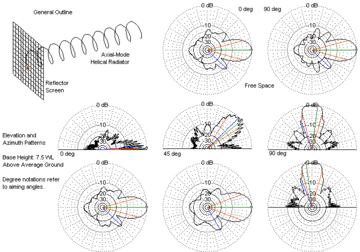
General Outline and Sample Patterns at Selected Angles 10-Turn, 1.15\lambda Circumference, 12-Degree Pitch Axial-Mode Helical Radiator
