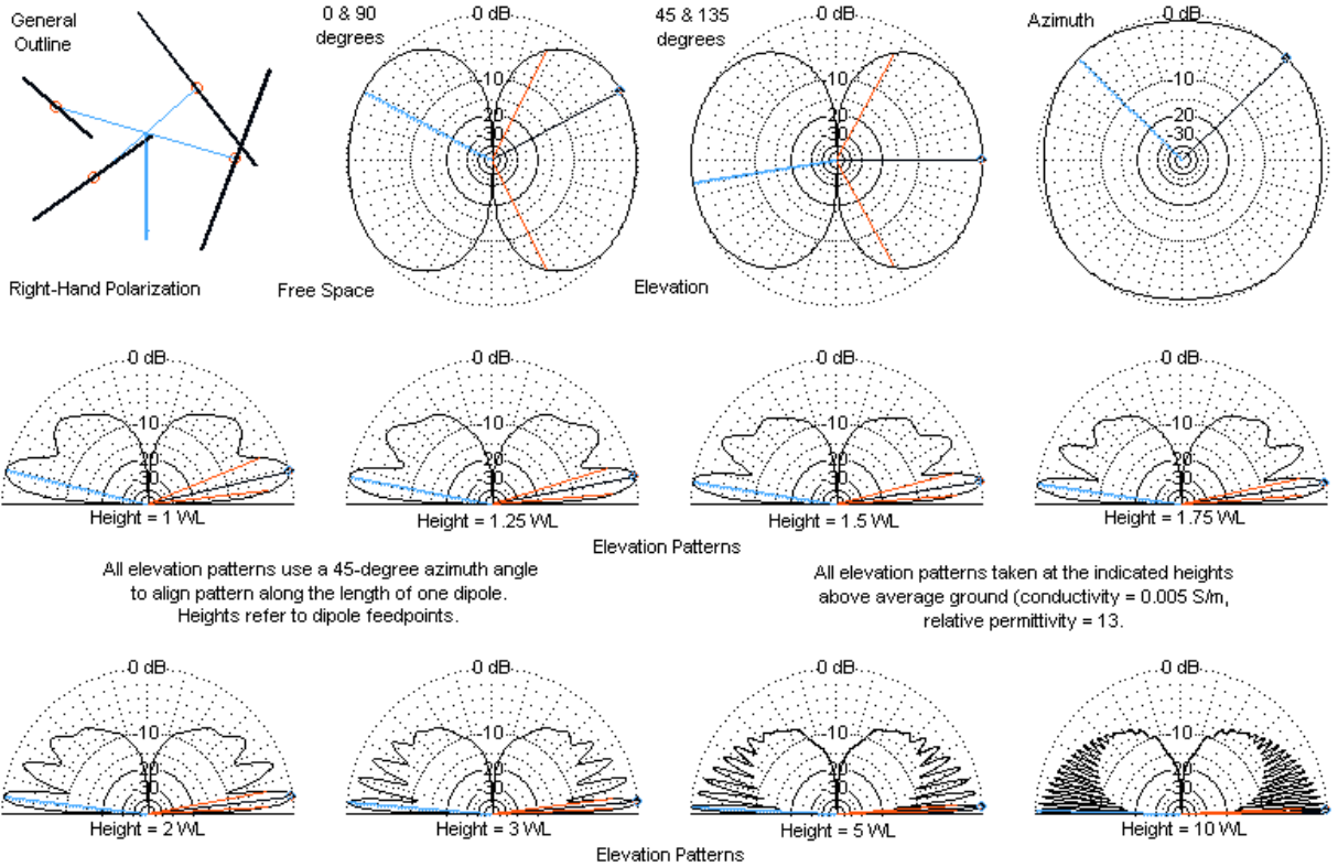
Sample Total-Field Patterns of a Right-Hand Polarized Original Lindenblad Array
