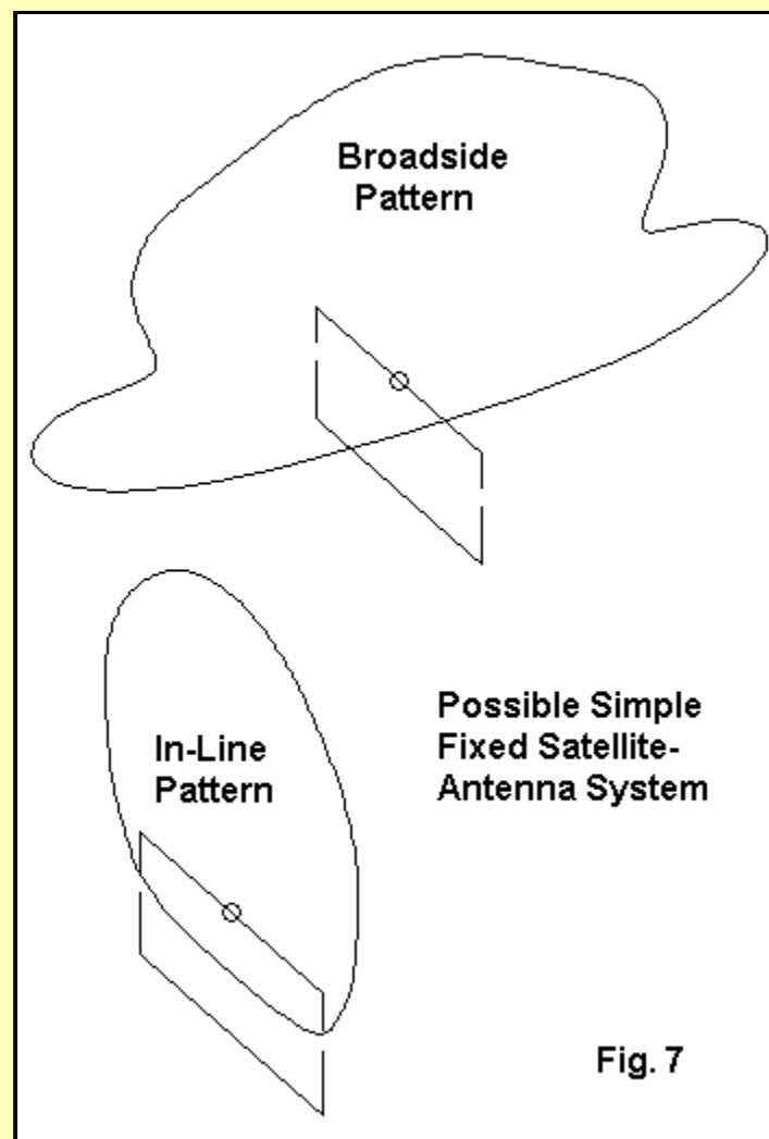
Fig. 7 shows the general outlines of the elevation patterns of the rectangle both broadside to the antenna and in-line with the wires. The 3-dimensional pattern makes a kind of tunnel across the
