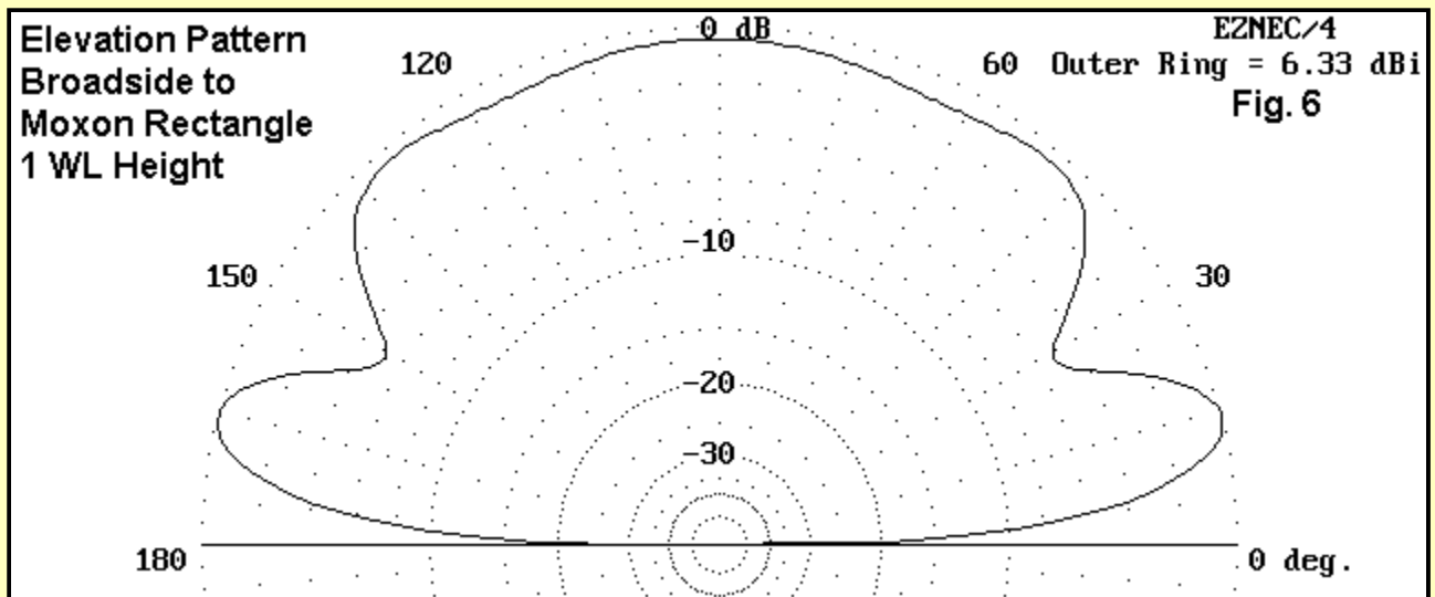
Fig. 6 shows the elevation pattern broadside to a 2-meter Moxon rectangle that is 1 wl off the ground. Although each side of the pattern shows a null, the remaining curve is remarkably smooth and with roughly equal gain from one side to the other.
