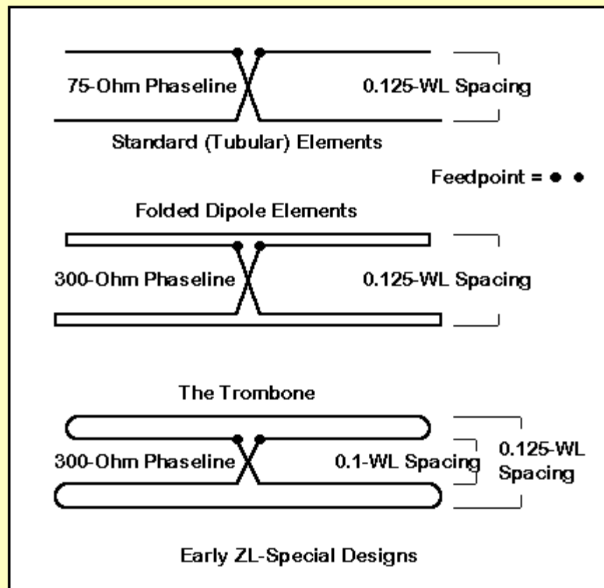
Fig. 3-1. Outline sketches of several classic ZL-Special designs.
