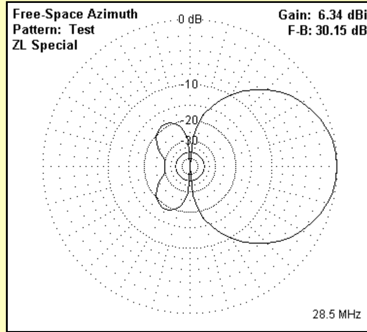
Fig. 3-4. Free-space azimuth pattern of the sample ZL-Special at 28.5 MHz.
