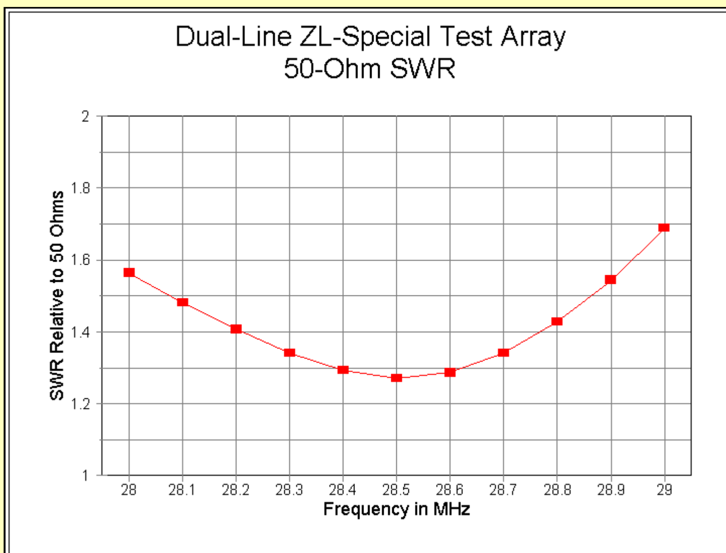
Fig. 3-15. 50-Ohm SWR curve of the dual-line ZL-Special from 28.0 to 29.0 MHz.
