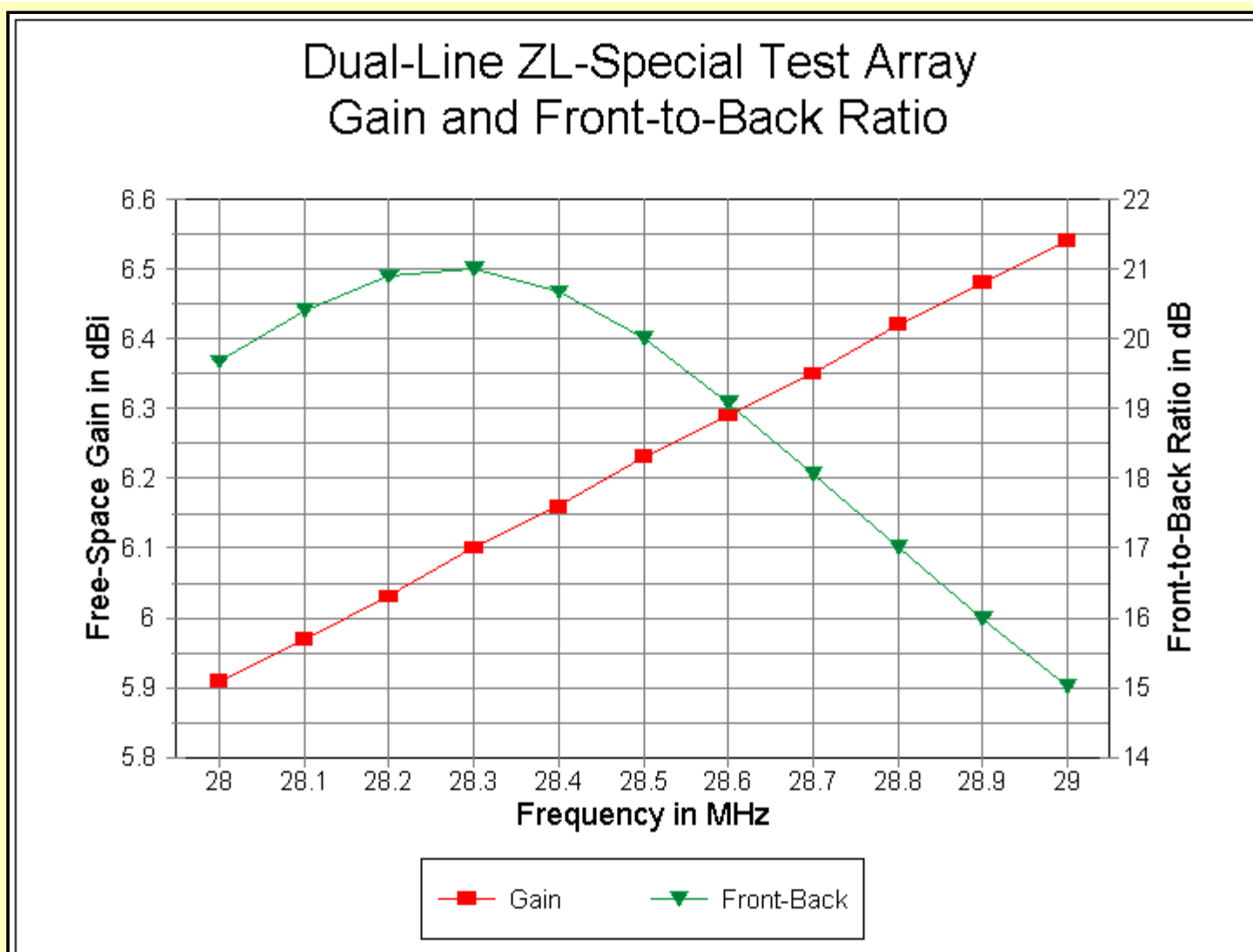
Fig. 3-14. Gain and 180° front-to-back ratio of the dual-line ZL-Special from 28.0 to 29.0 MHz.
