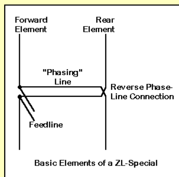
Fig. 3-2. The basic elements of a ZL-Special 2-element horizontal phased array.
