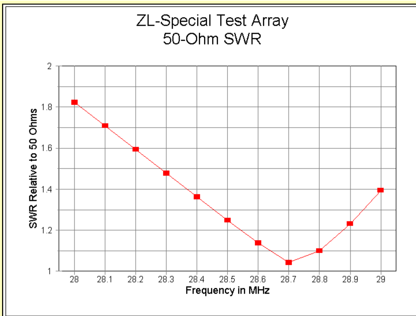
Fig. 3-6. 50-Ohm SWR curve of the sample ZL-Special from 28.0 to 29.0 MHz.
