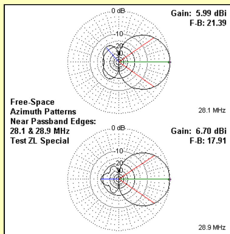
Fig. 3-7. Free-space azimuth patterns of the sample ZL-Special at 28.1 and 28.9 MHz.
