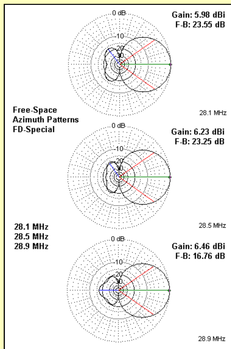
3-9. Free-space azimuth patterns of the Field-Day Special at 28.1, 28.5, and 28.9 MHz.
