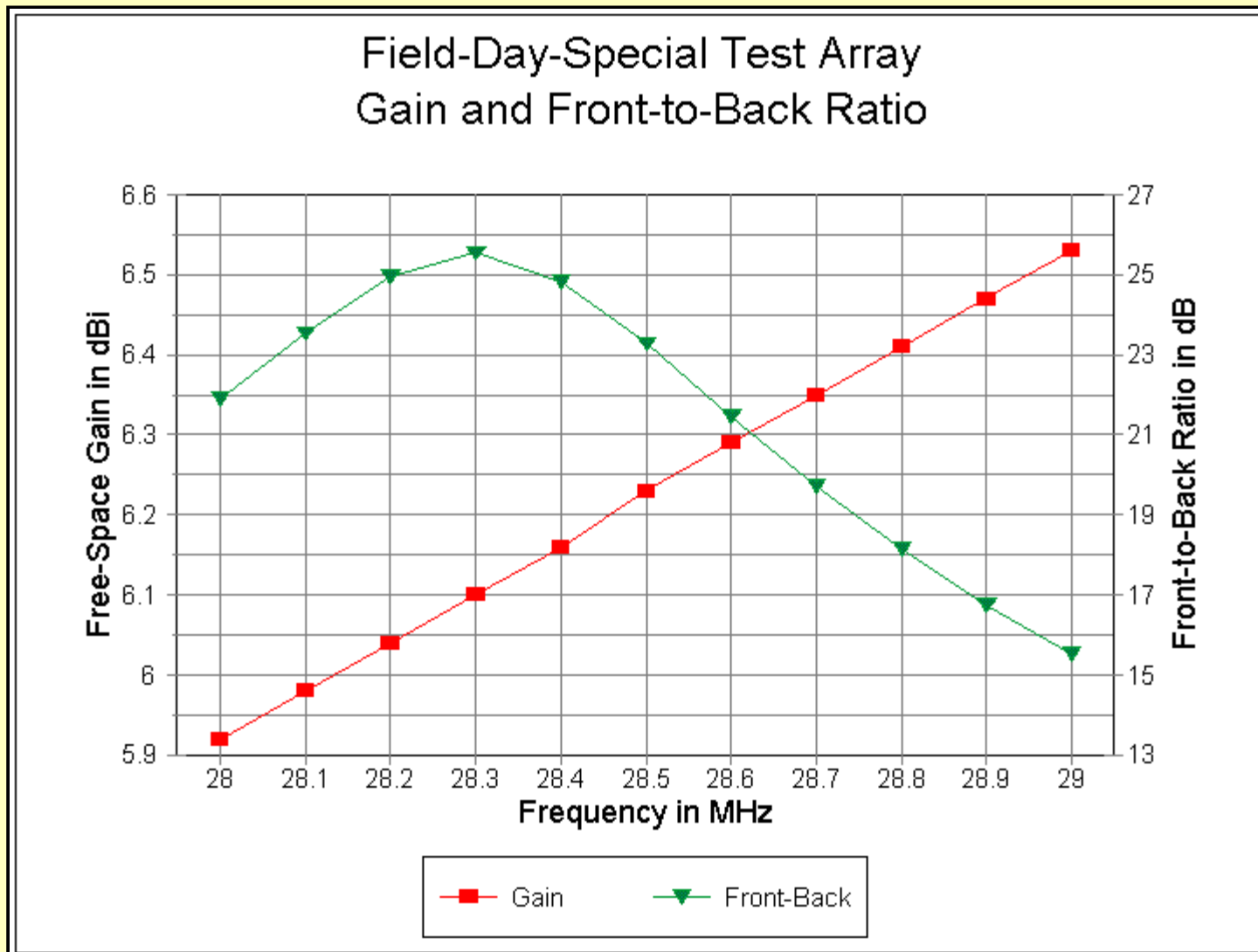
Fig. 3-10. Gain and 180° front-to-back ratio of the Field-Day Special from 28.0 to 29.0 MHz.
