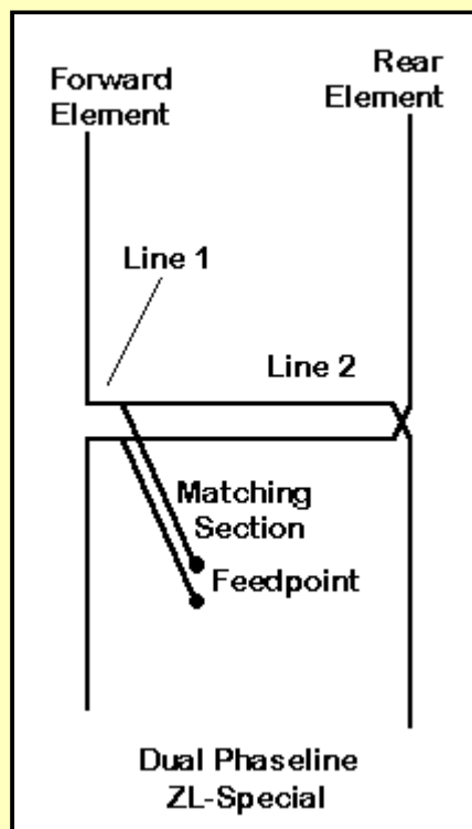
Fig. 3-12. Basic outline of the dual-line ZL-Special for 28.5 MHz.
