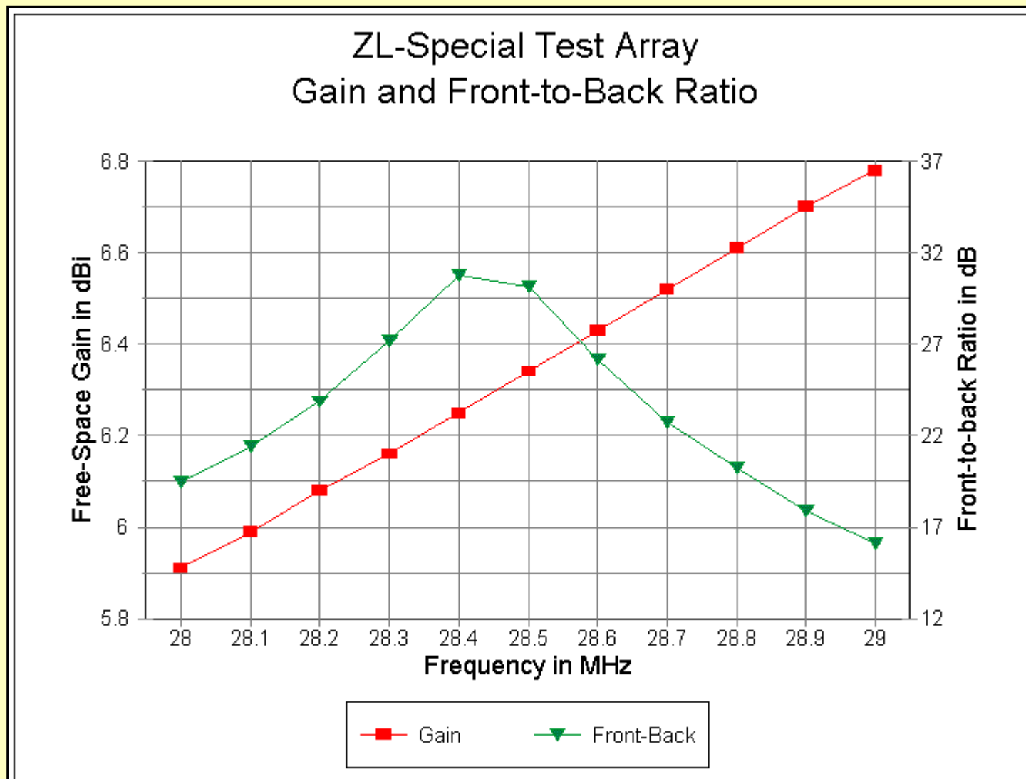
Fig.3-5. Gain and 180° front-to-back ratio of the sample ZL-Special from 28.0 to 29.0 MHz.
