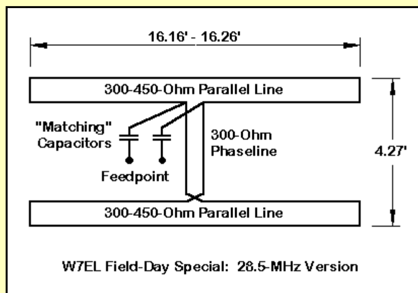
Fig. 3-8. Basic outline of a W7EL Field-Day Special for 28.5 MHz.
