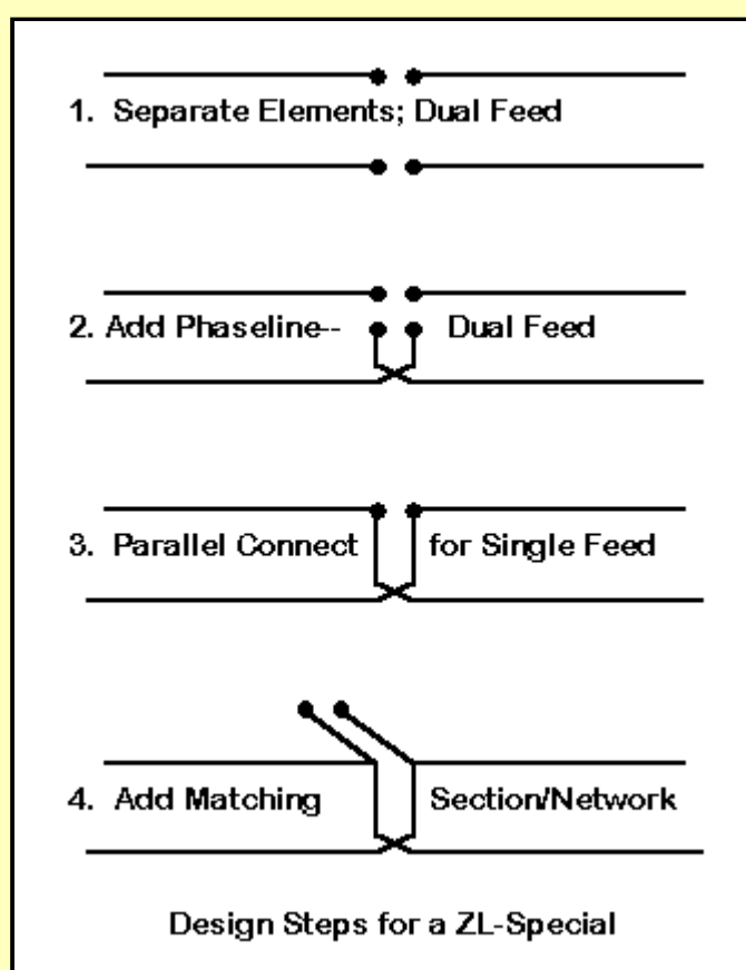
Fig. 3-3. Design steps for a ZL-Special used for array analysis.
