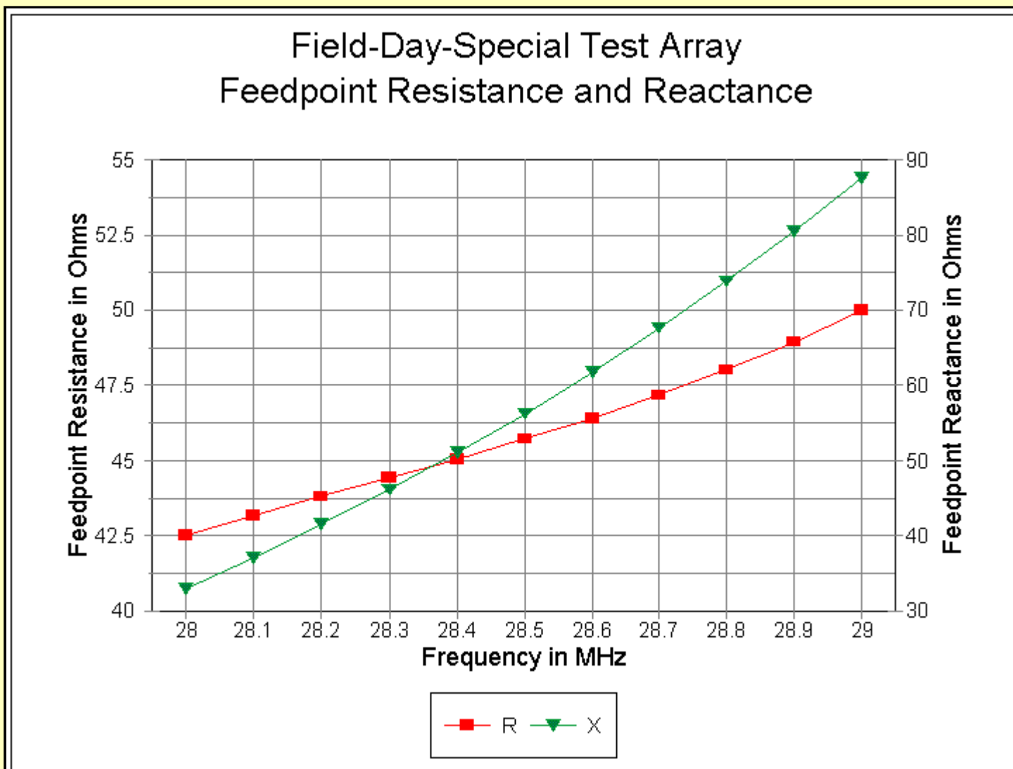
Fig. 3-11. Source resistance and reactance of the Field-Day Special from 28.0 to 29.0 MHz.
