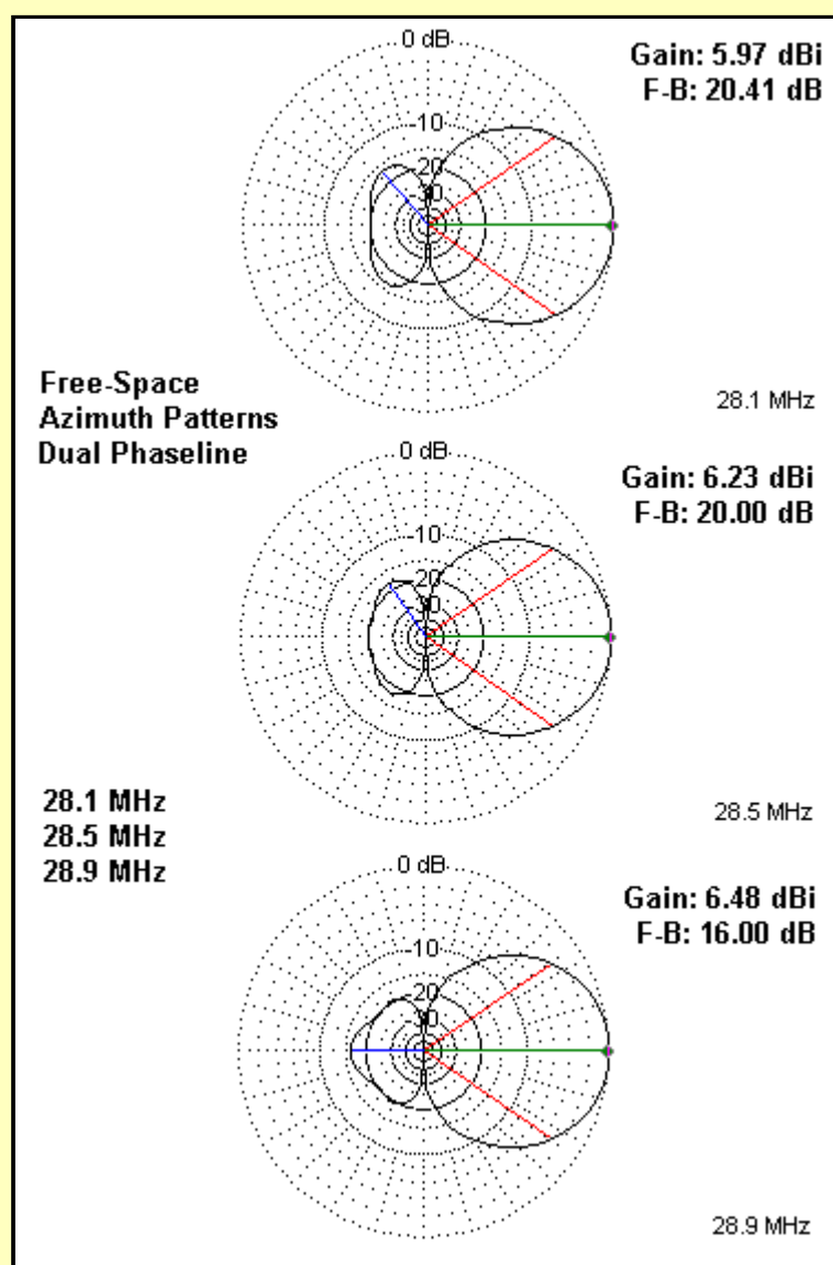
Fig. 3-13. Free-space azimuth pattern of the dual-line ZL-Special at 28.1, 28.5, and 28.9 MHz.
